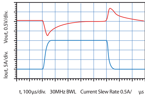
TRANSIENT RESPONSE, V_{in}=300V, I_{out}=5A-20A-5A, T_c=25^\circ C
