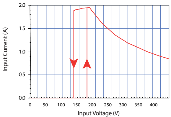
INPUT CHARACTERISTIC, I_{out} = 25A, T_c=25^\circ C
